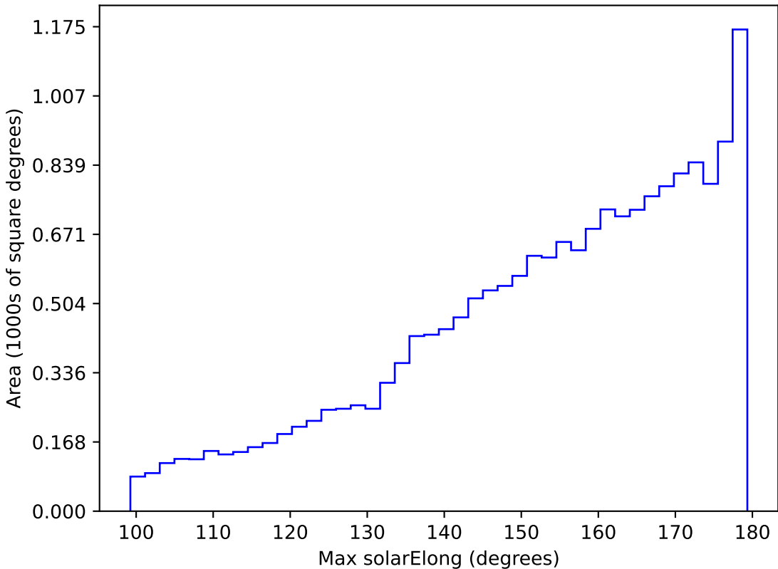
weather_cloudso10v3.4_10yrs WFD z band: Max solarElong
