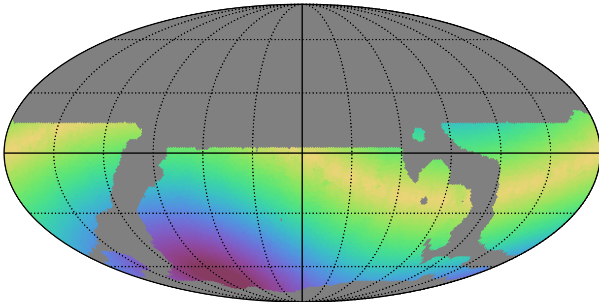
weather_cloudso10v3.4_10yrs WFD u band: Max solarElong
