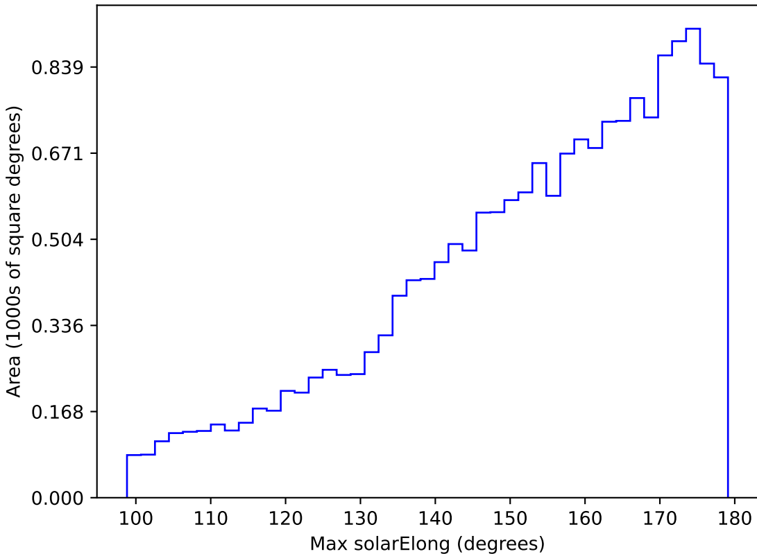
weather_cloudso10v3.4_10yrs WFD u band: Max solarElong
