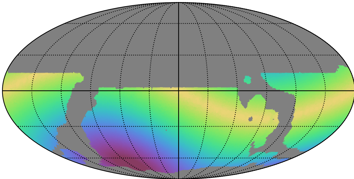
weather_cloudso10v3.4_10yrs WFD r band: Max solarElong
