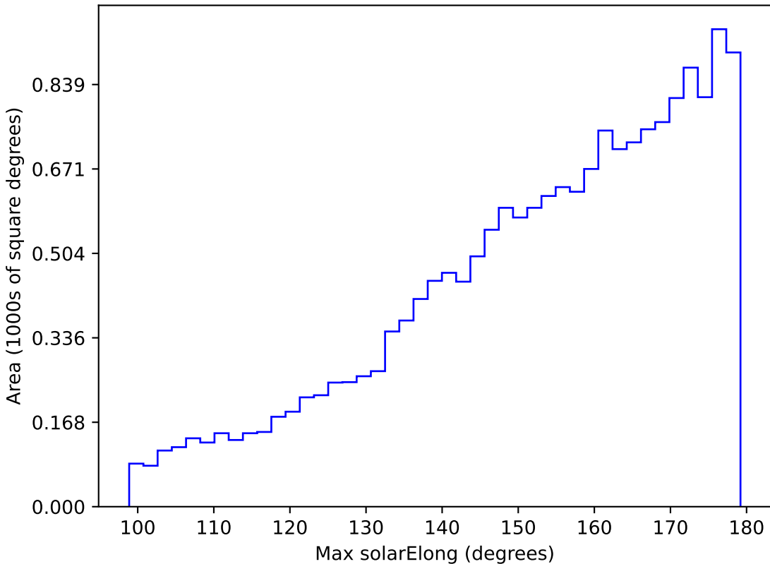
weather_cloudso10v3.4_10yrs WFD g band: Max solarElong
