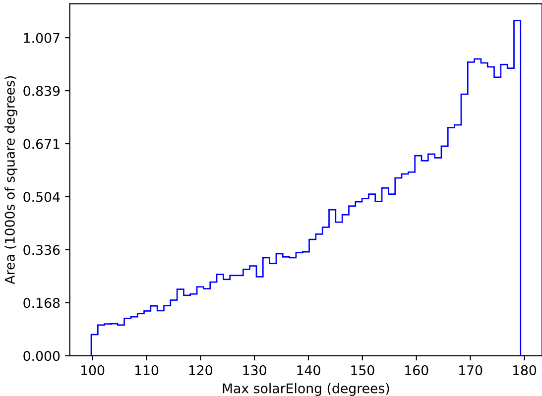
weather_cloudso10v3.4_10yrs All sky z band: Max solarElong
