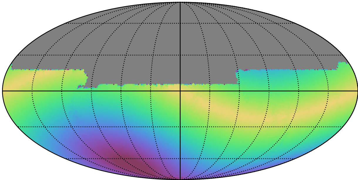
weather_cloudso10v3.4_10yrs All sky y band: Max solarElong
