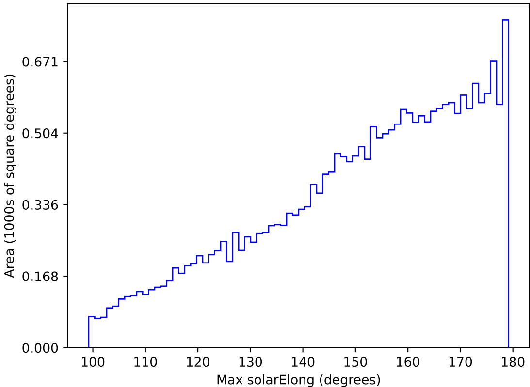
weather_cloudso10v3.4_10yrs All sky y band: Max solarElong
