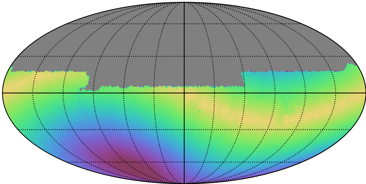
weather_cloudso10v3.4_10yrs All sky u band: Max solarElong
