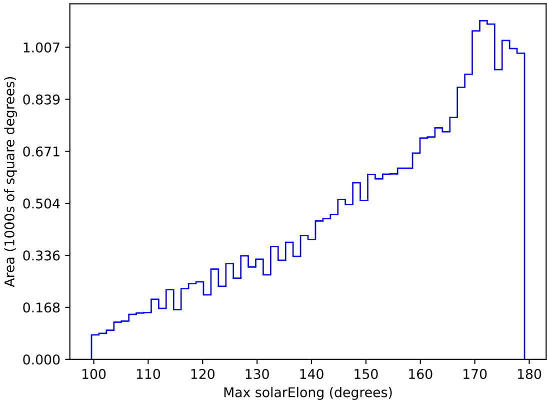
weather_cloudso10v3.4_10yrs All sky g band: Max solarElong
