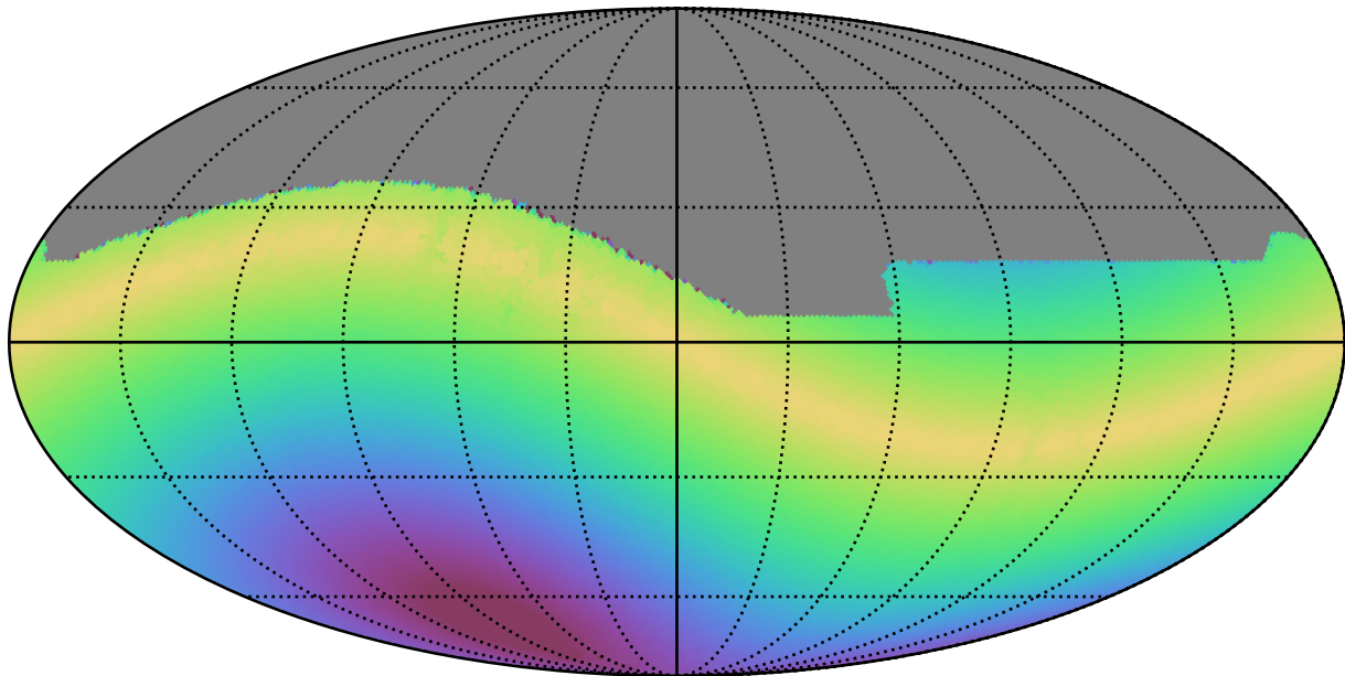
weather_cloudso10v3.4_10yrs All sky all bands: Max solarElong
