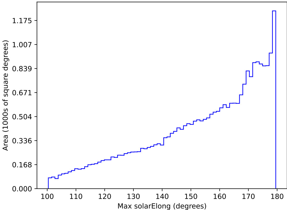
weather_cloudso10v3.4_10yrs All sky all bands: Max solarElong
