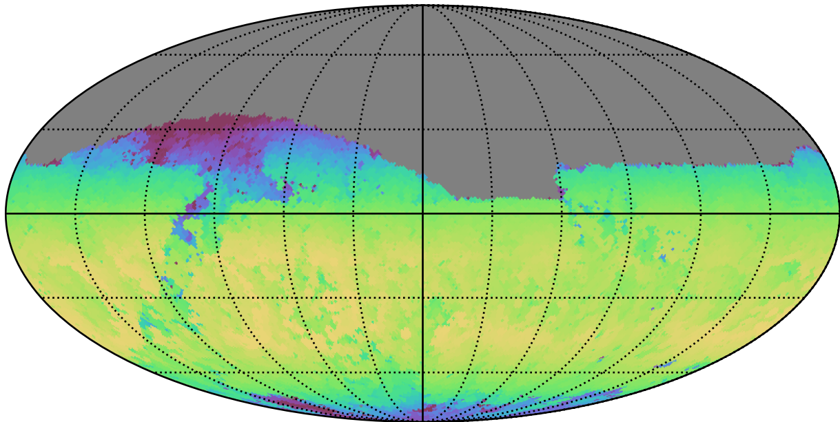
weather_cloudso10v3.4_10yrs Yr 1 z band: Max skyBrightness
