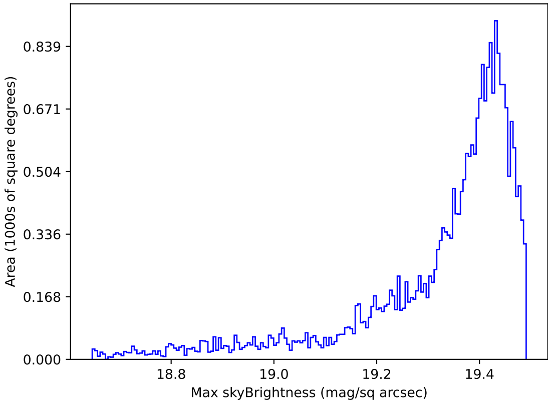
weather_cloudso10v3.4_10yrs Yr 1 z band: Max skyBrightness
