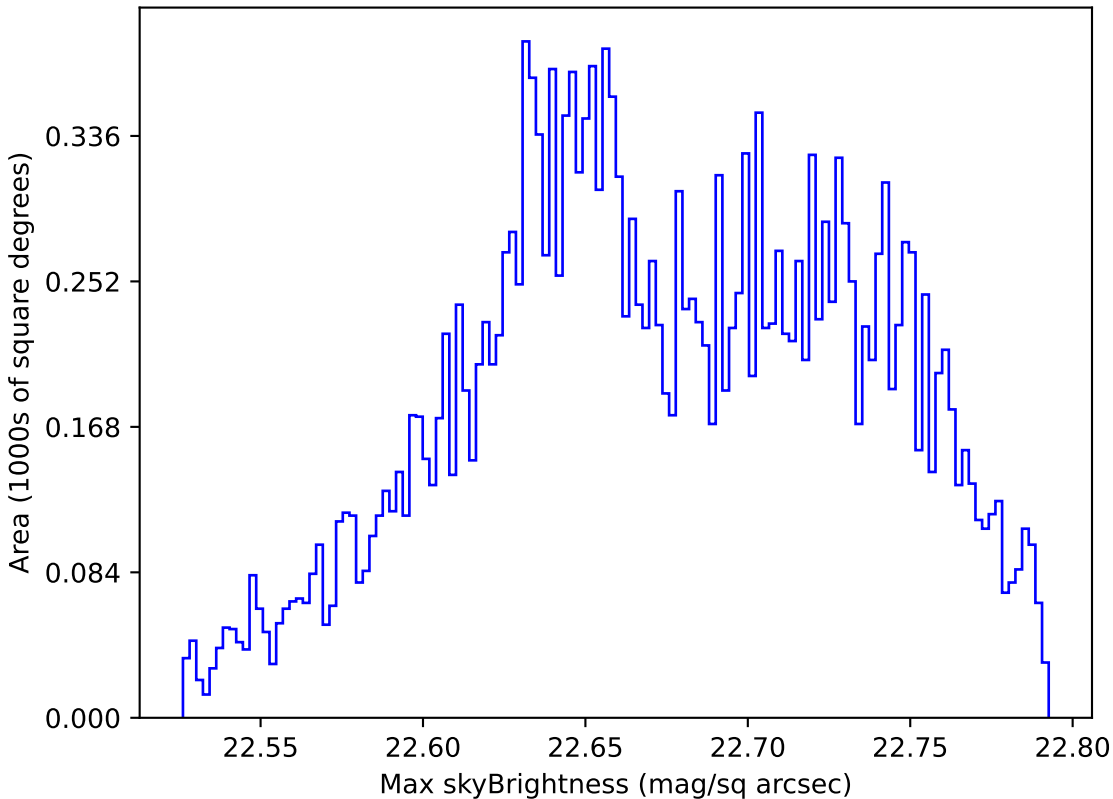
weather_cloudso10v3.4_10yrs Yr 1 u band: Max skyBrightness
