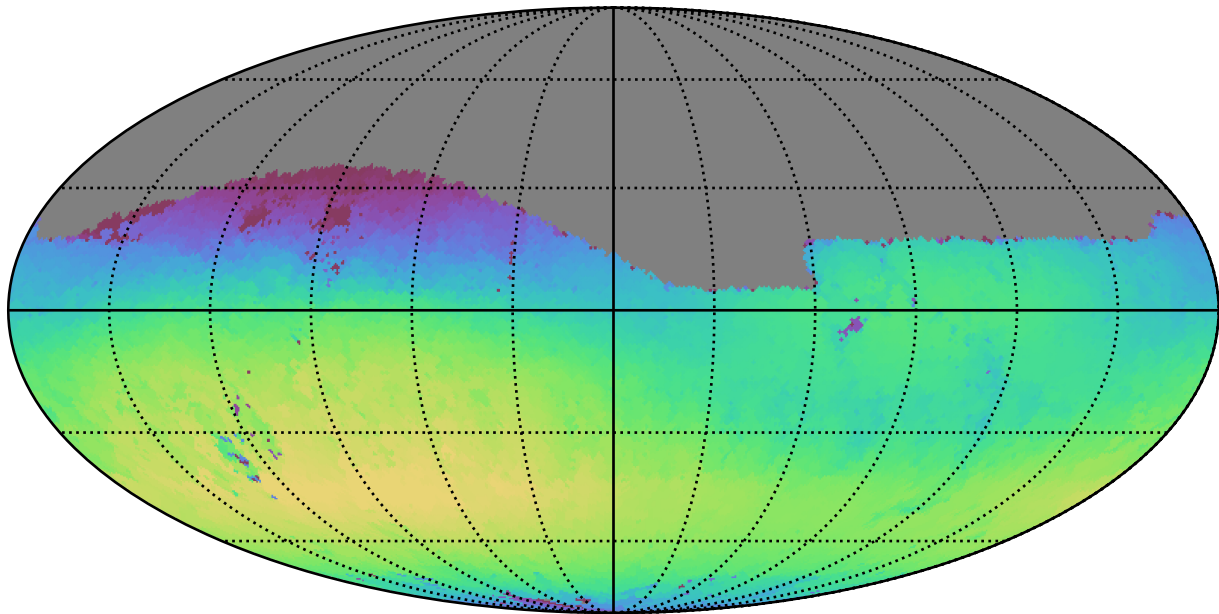
weather_cloudso10v3.4_10yrs Yr 1 r band: Max skyBrightness
