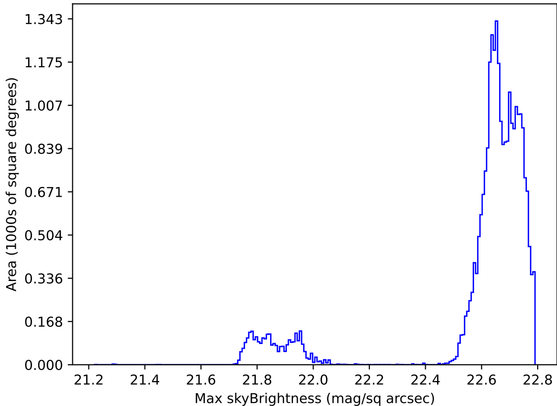
weather_cloudso10v3.4_10yrs Yr 1 all bands: Max skyBrightness
