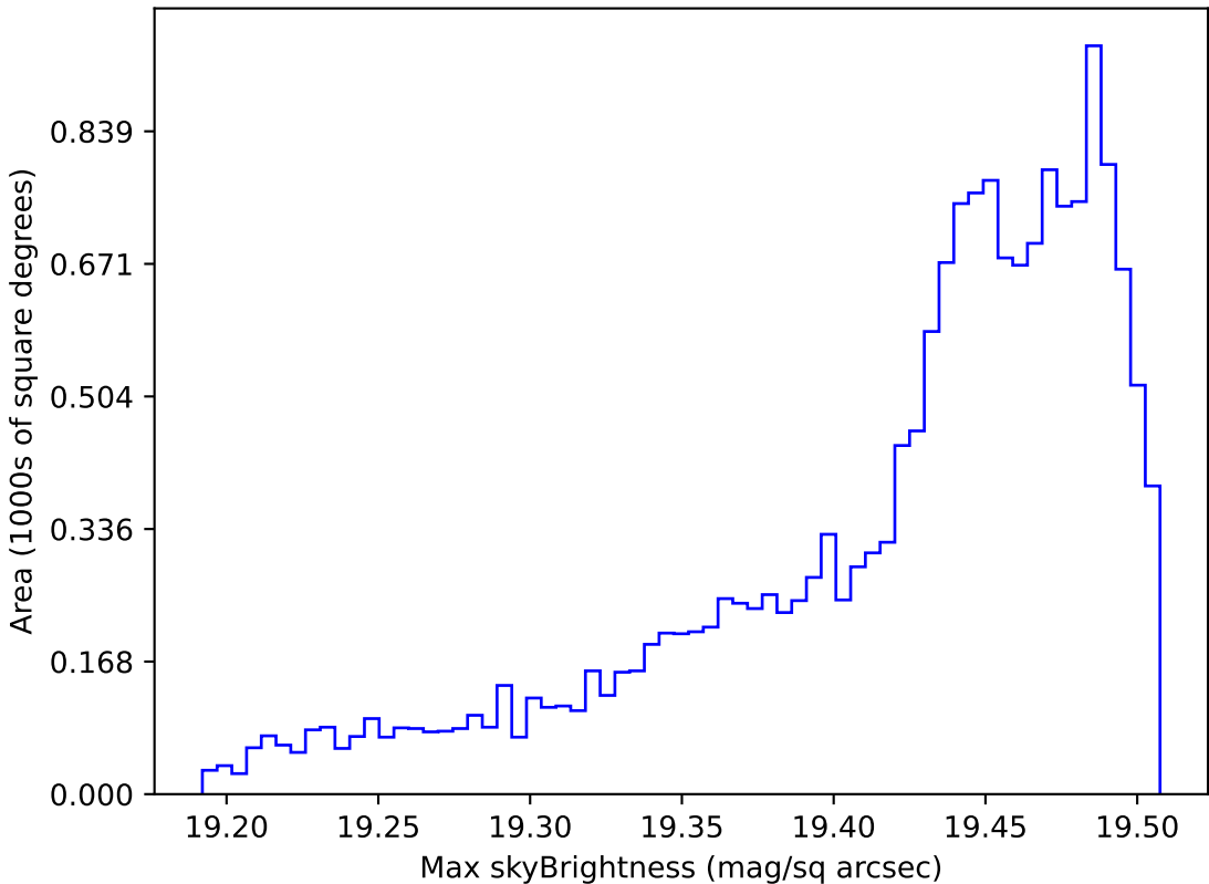
weather_cloudso10v3.4_10yrs WFD z band: Max skyBrightness
