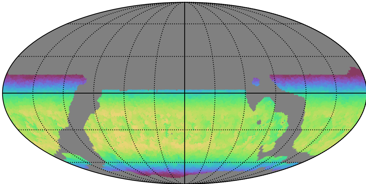
weather_cloudso10v3.4_10yrs WFD y band: Max skyBrightness
