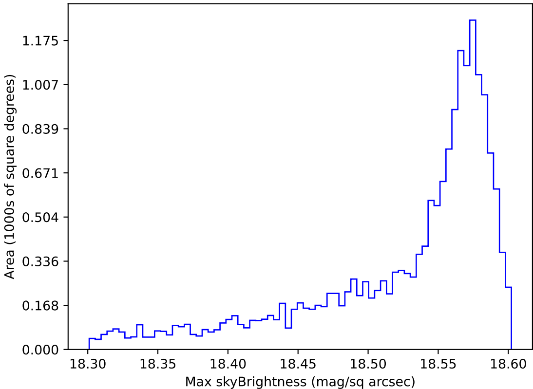
weather_cloudso10v3.4_10yrs WFD y band: Max skyBrightness
