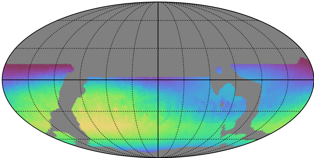
weather_cloudso10v3.4_10yrs WFD u band: Max skyBrightness
