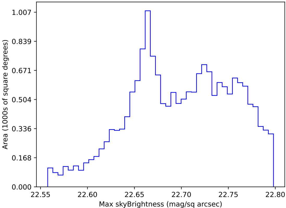
weather_cloudso10v3.4_10yrs WFD u band: Max skyBrightness
