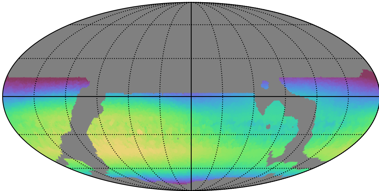
weather_cloudso10v3.4_10yrs WFD i band: Max skyBrightness
