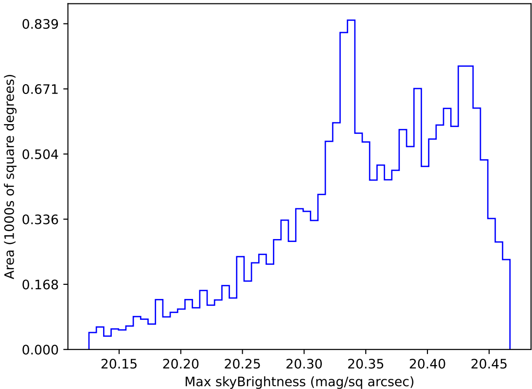
weather_cloudso10v3.4_10yrs WFD i band: Max skyBrightness
