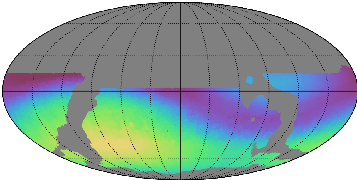
weather_cloudso10v3.4_10yrs WFD g band: Max skyBrightness
