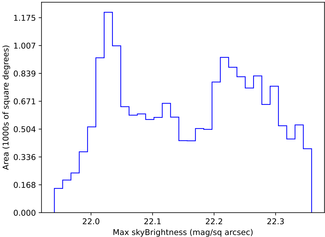
weather_cloudso10v3.4_10yrs WFD g band: Max skyBrightness
