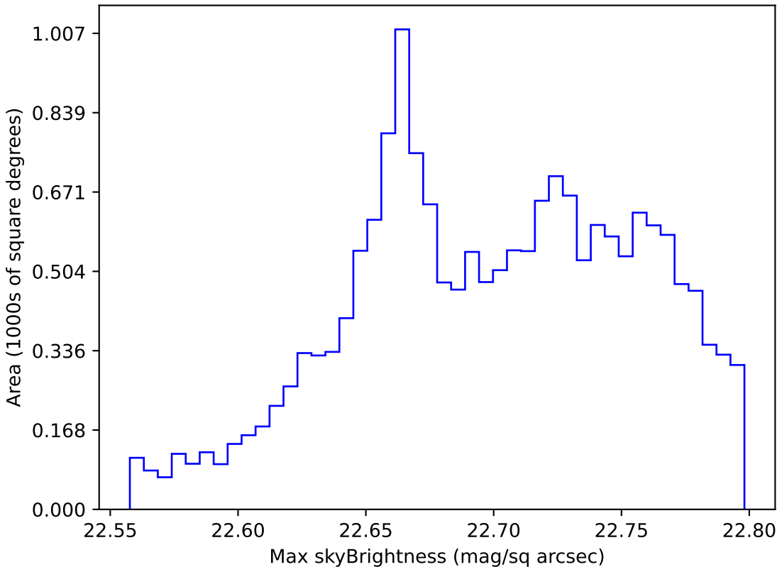
weather_cloudso10v3.4_10yrs WFD all bands: Max skyBrightness
