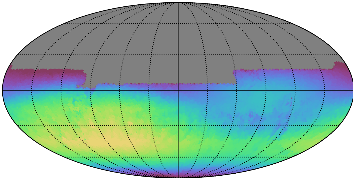
weather_cloudso10v3.4_10yrs All sky u band: Max skyBrightness
