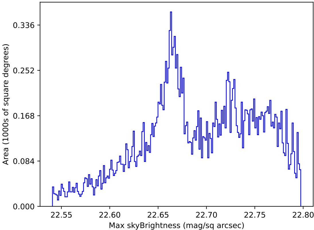
weather_cloudso10v3.4_10yrs All sky u band: Max skyBrightness
