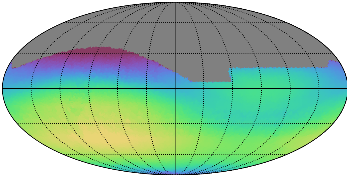
weather_cloudso10v3.4_10yrs All sky r band: Max skyBrightness
