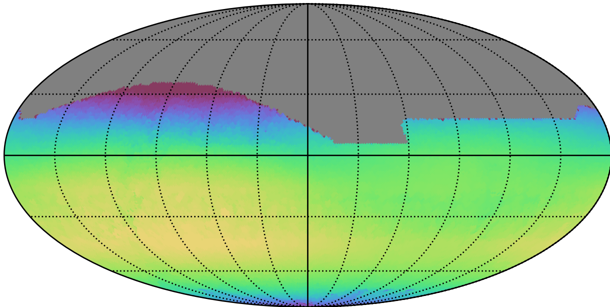
weather_cloudso10v3.4_10yrs All sky i band: Max skyBrightness
