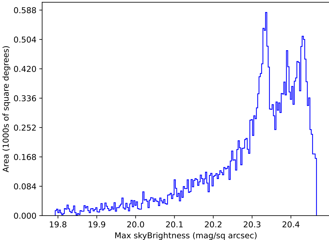
weather_cloudso10v3.4_10yrs All sky i band: Max skyBrightness
