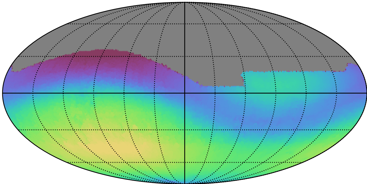
weather_cloudso10v3.4_10yrs All sky g band: Max skyBrightness
