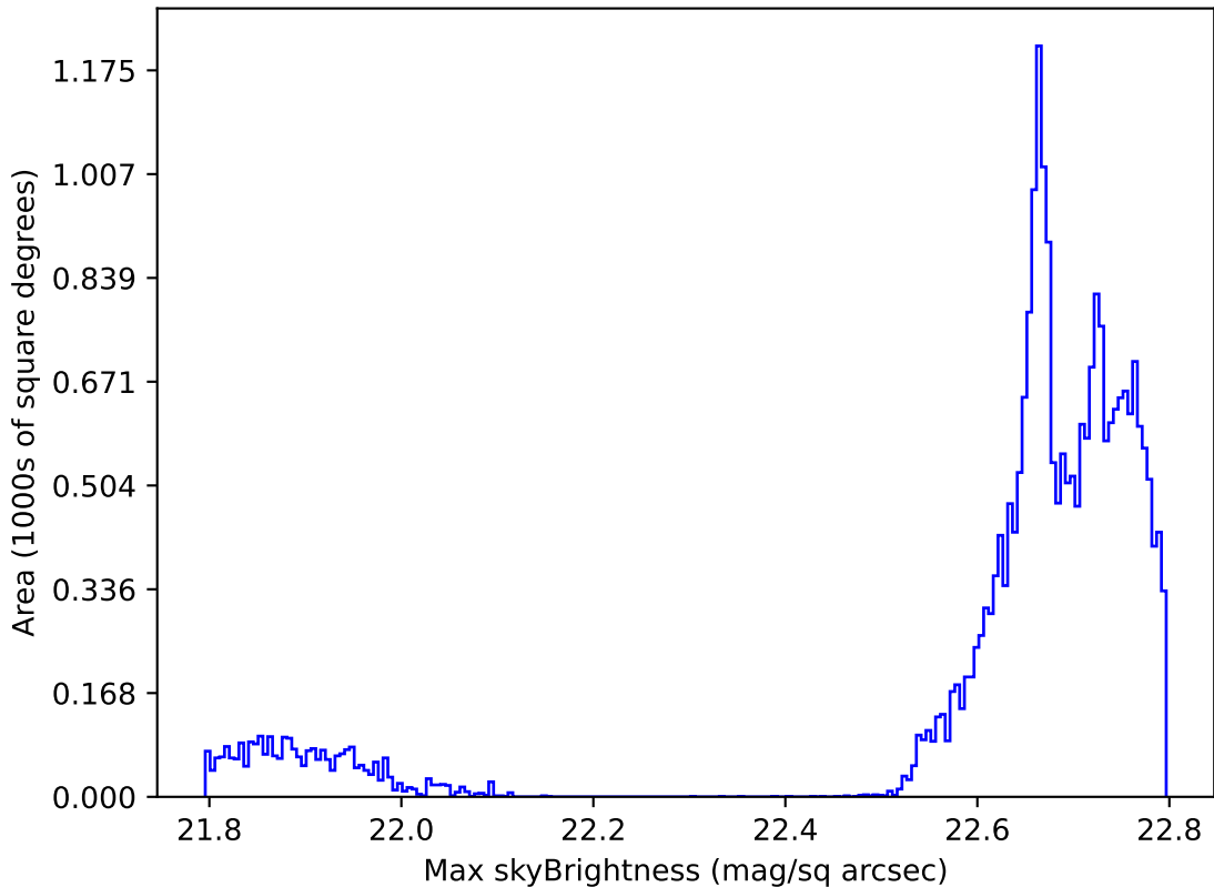
weather_cloudso10v3.4_10yrs All sky all bands: Max skyBrightness
