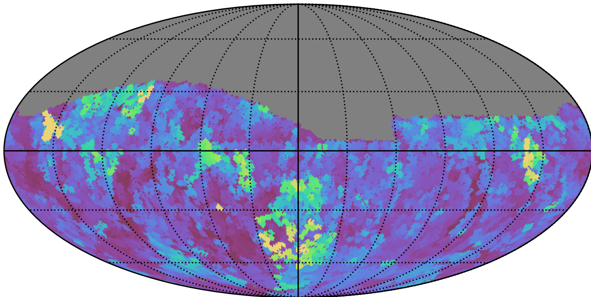
weather_cloudso10v3.4_10yrs Yr 1 z band: Max seeingGeom
