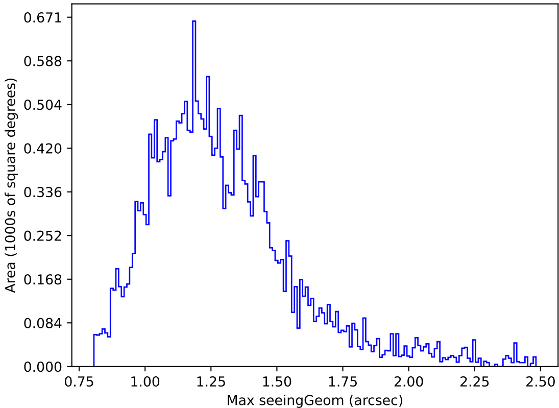
weather_cloudso10v3.4_10yrs Yr 1 z band: Max seeingGeom
