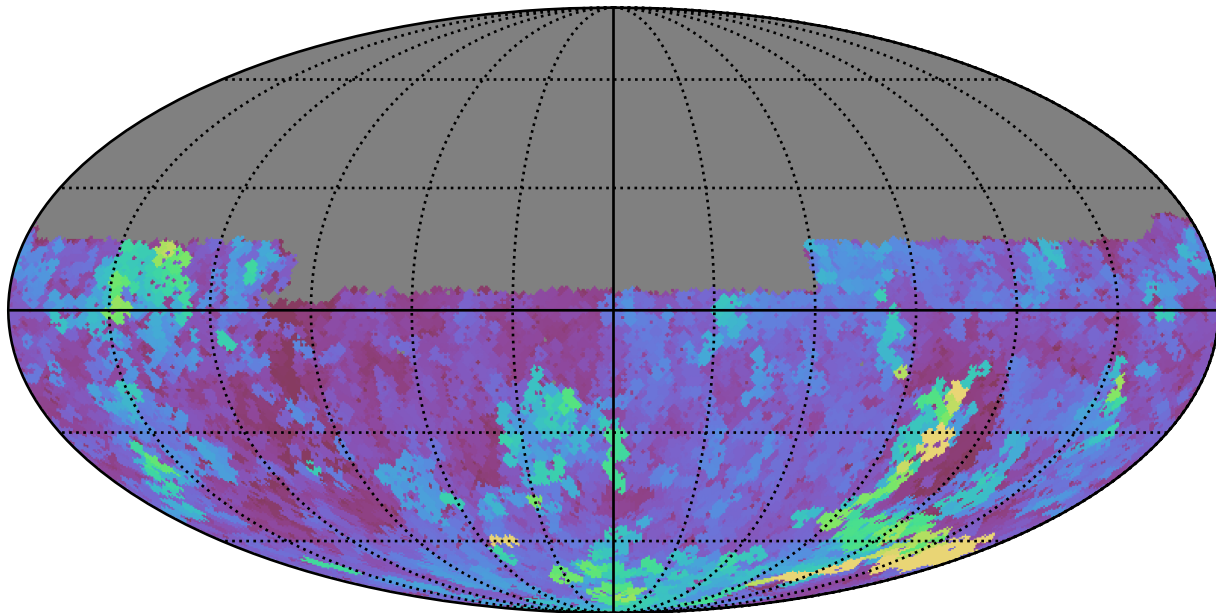
weather_cloudso10v3.4_10yrs Yr 1 u band: Max seeingGeom
