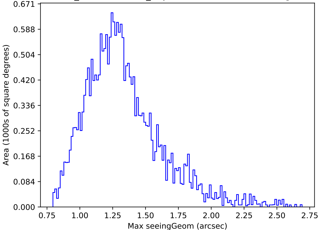
weather_cloudso10v3.4_10yrs Yr 1 u band: Max seeingGeom
