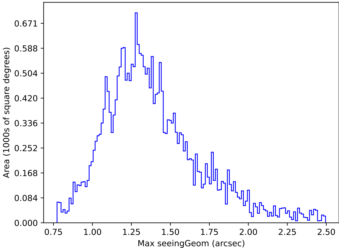
weather_cloudso10v3.4_10yrs Yr 1 r band: Max seeingGeom
