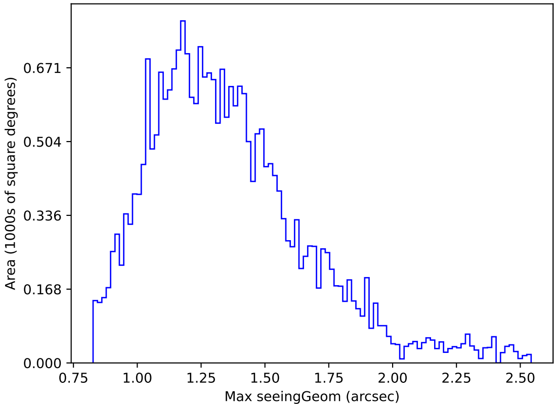
weather_cloudso10v3.4_10yrs Yr 1 i band: Max seeingGeom
