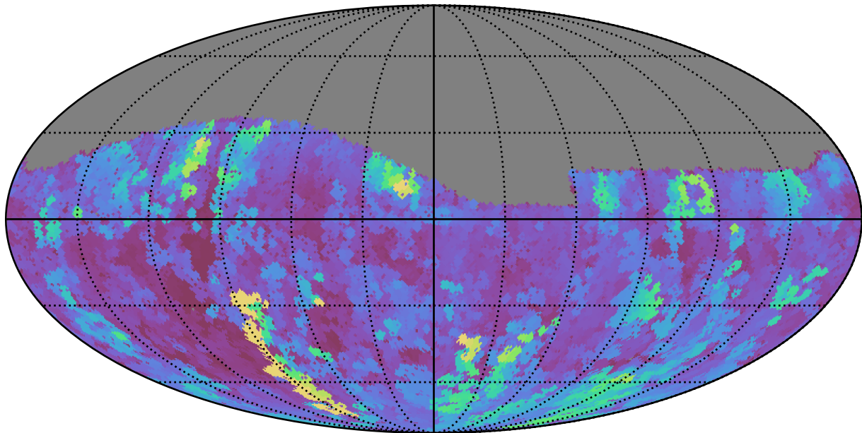
weather_cloudso10v3.4_10yrs Yr 1 g band: Max seeingGeom
