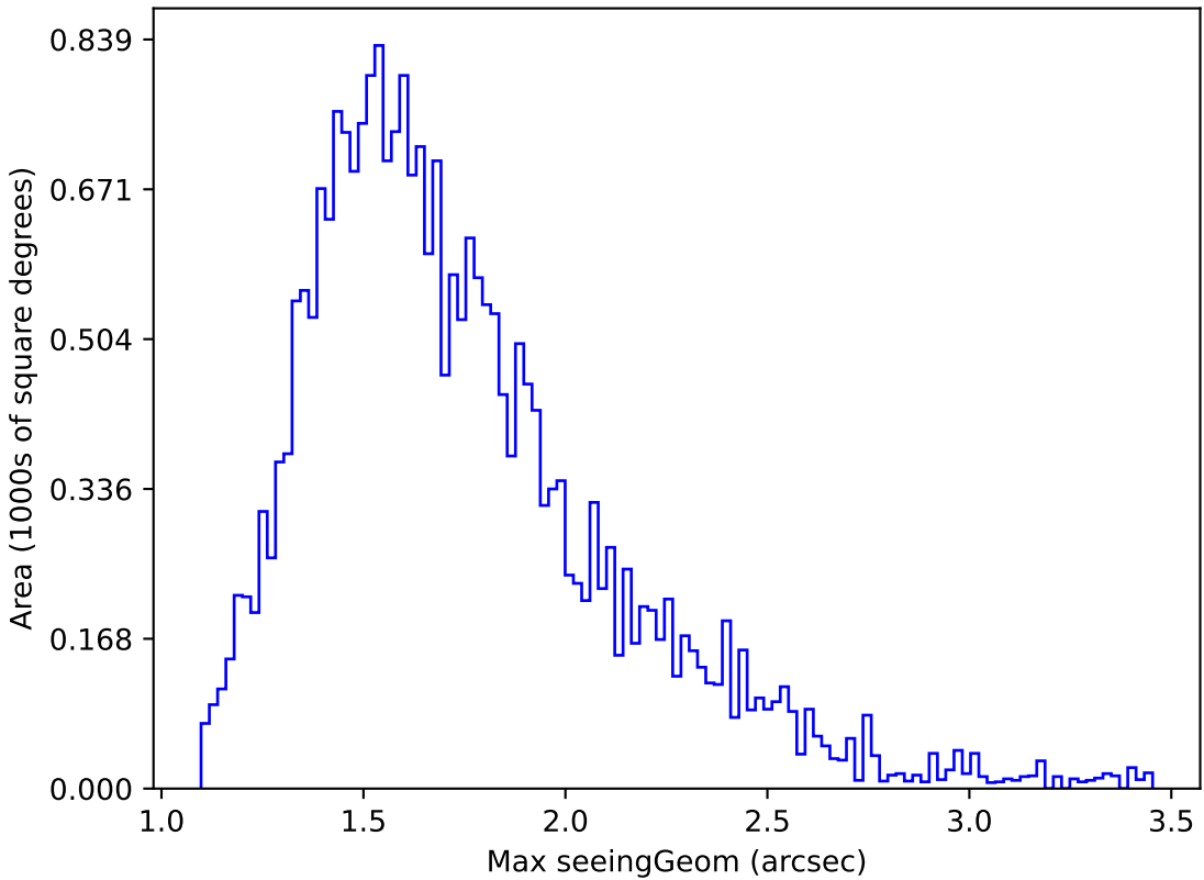
weather_cloudso10v3.4_10yrs Yr 1 all bands: Max seeingGeom
