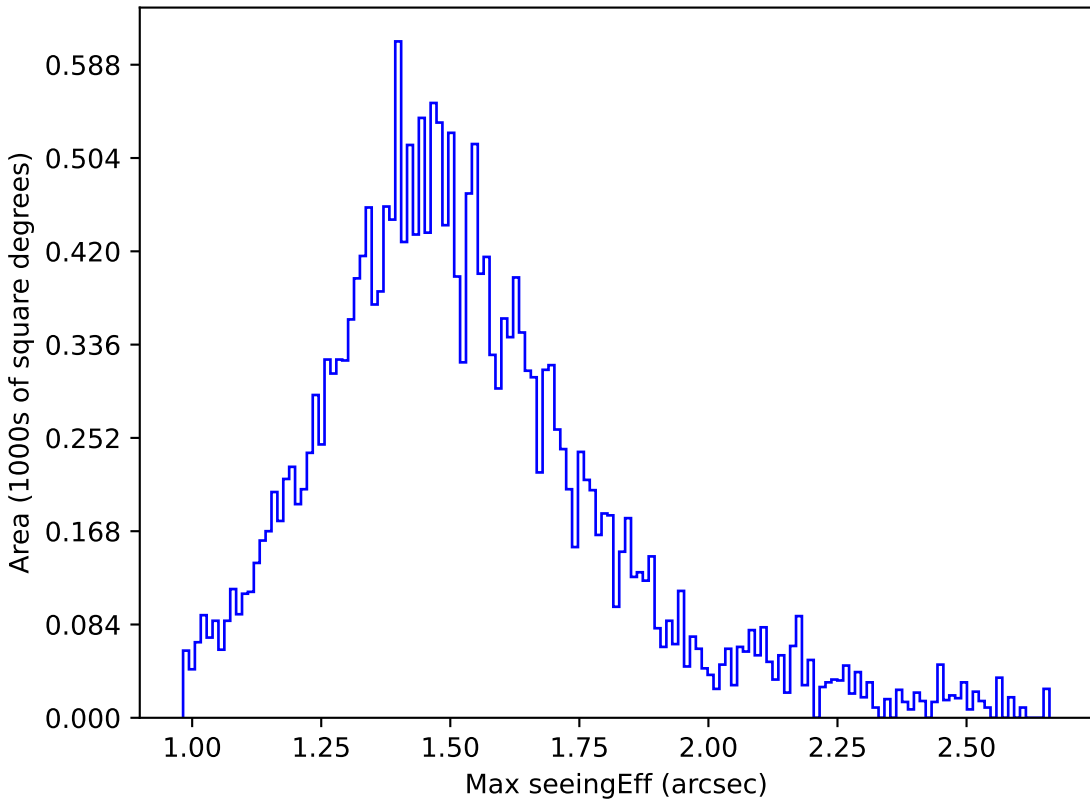
weather_cloudso10v3.4_10yrs Yr 1 y band: Max seeingEff
