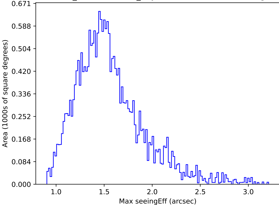
weather_cloudso10v3.4_10yrs Yr 1 u band: Max seeingEff
