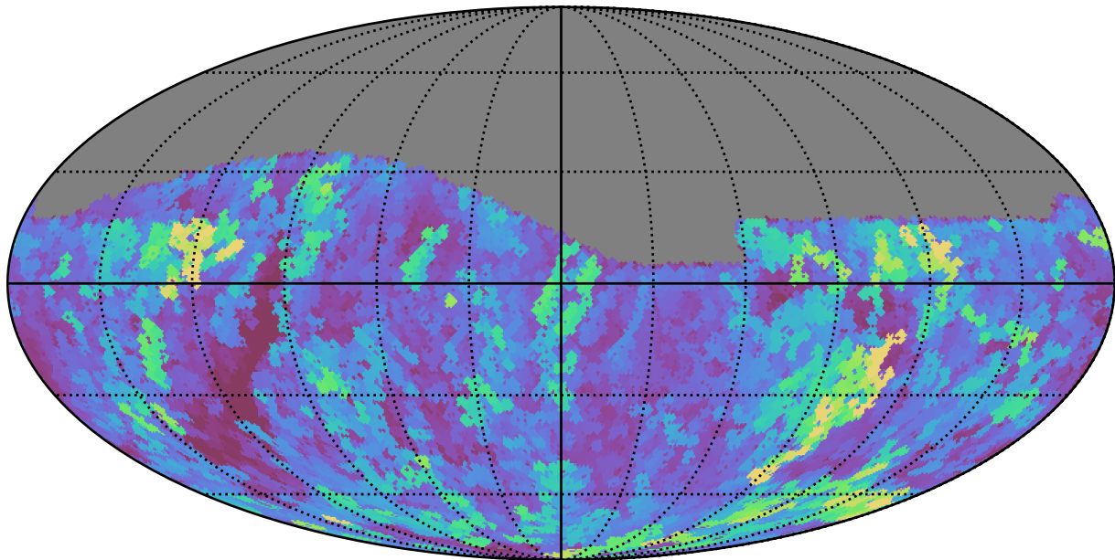
weather_cloudso10v3.4_10yrs Yr 1 r band: Max seeingEff
