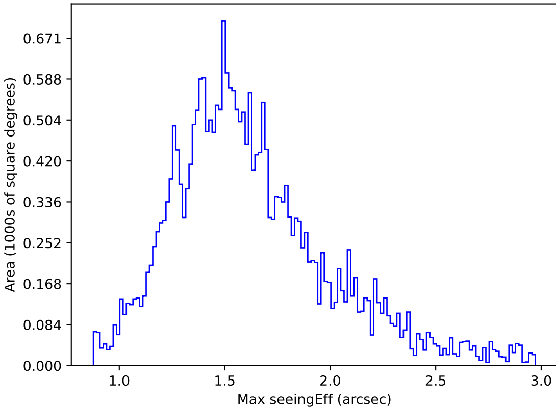
weather_cloudso10v3.4_10yrs Yr 1 r band: Max seeingEff
