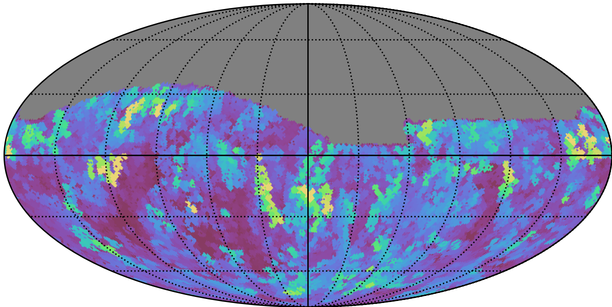
weather_cloudso10v3.4_10yrs Yr 1 i band: Max seeingEff
