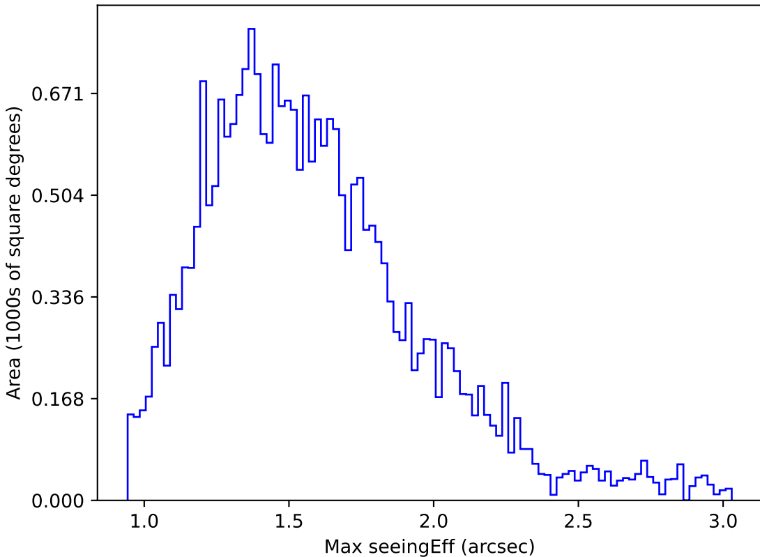
weather_cloudso10v3.4_10yrs Yr 1 i band: Max seeingEff
