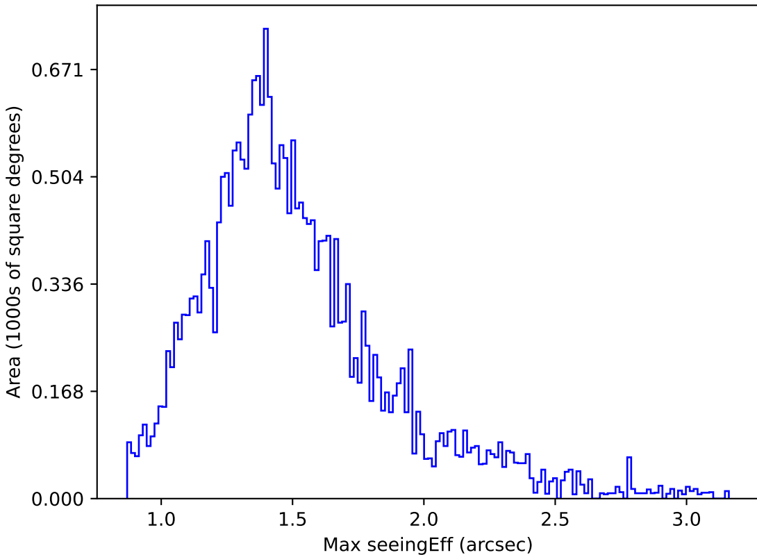
weather_cloudso10v3.4_10yrs Yr 1 g band: Max seeingEff
