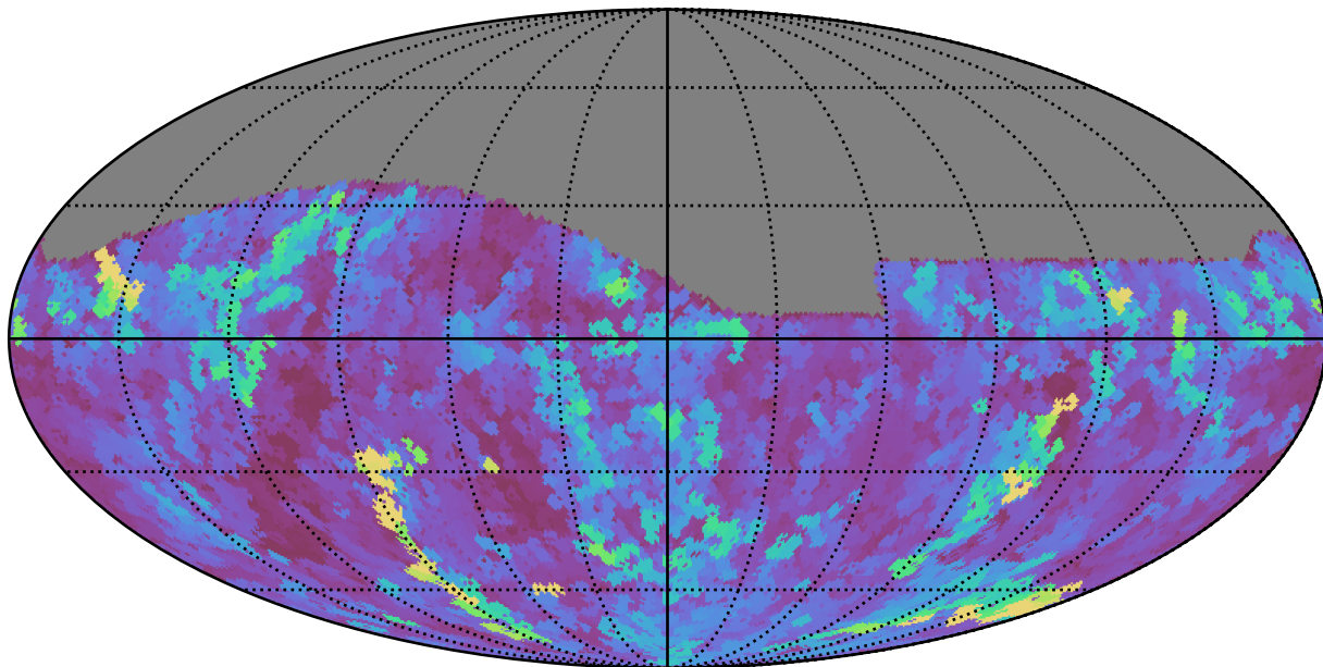
weather_cloudso10v3.4_10yrs Yr 1 all bands: Max seeingEff
